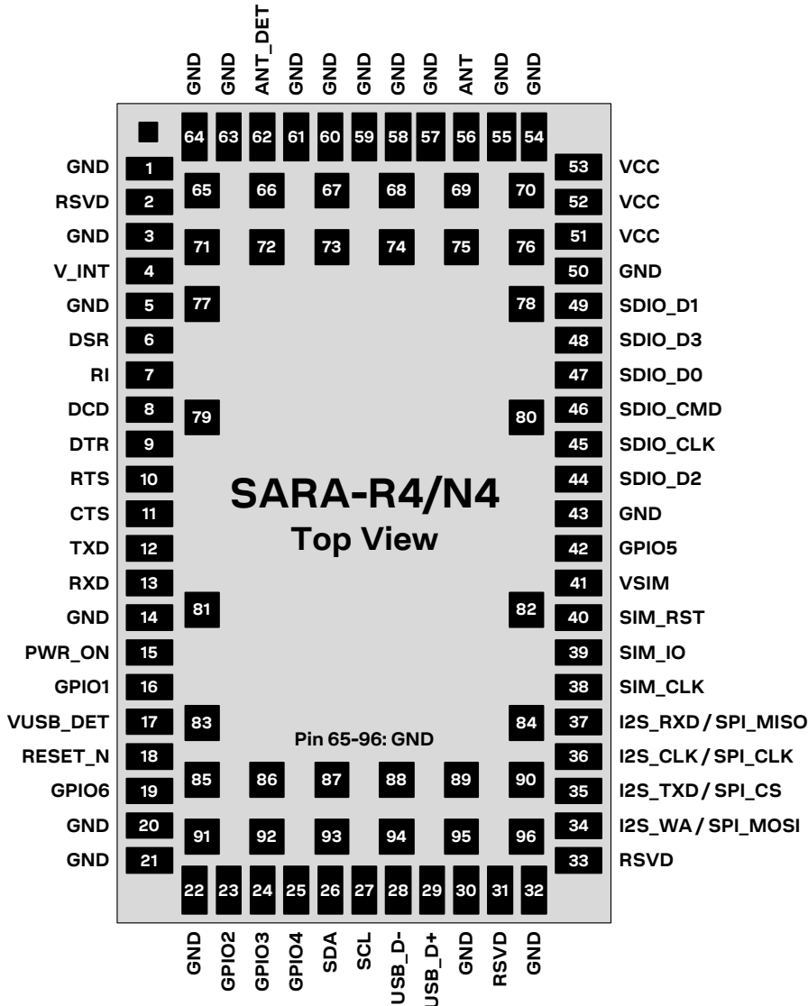
Figure 2: SARA-R4 series pin assignment (top view)
